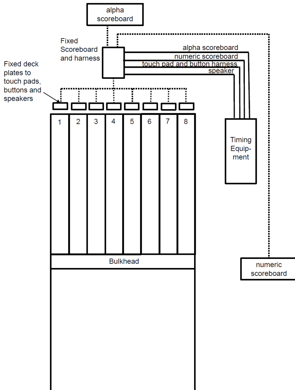
Figure 1: 8 Lanes Down the Pool Configuration.
