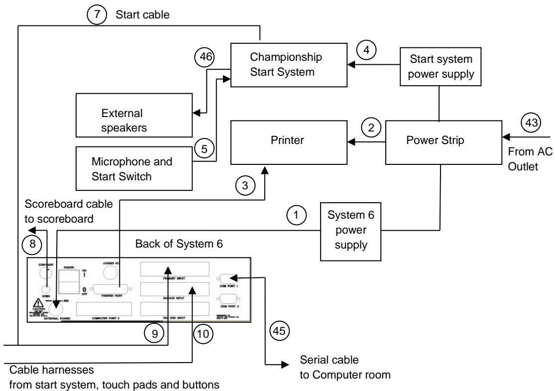
Figure 33: System 6 electrical connection diagram.
